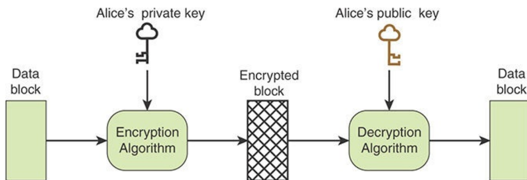
(c) Public-key encryption/decryption (Alice authenticates block for any recipient)
