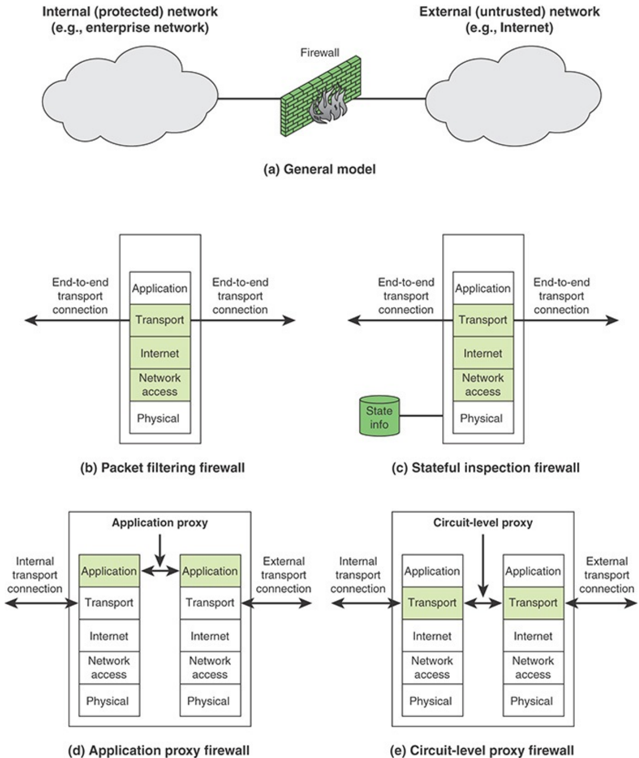
FIGURE 12.4 Types of Firewalls
