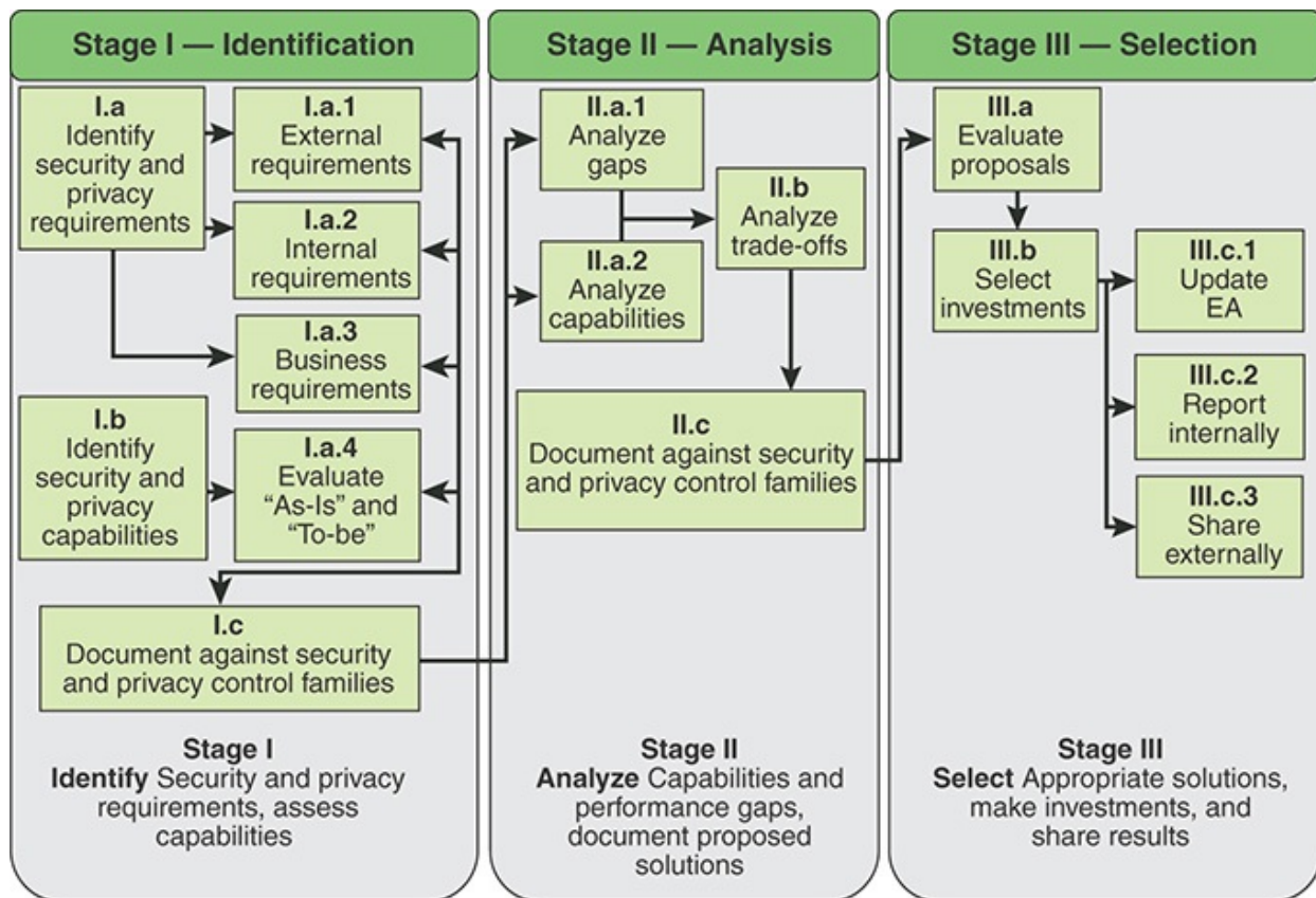
FIGURE 4.1 Example of a Security Planning Process
