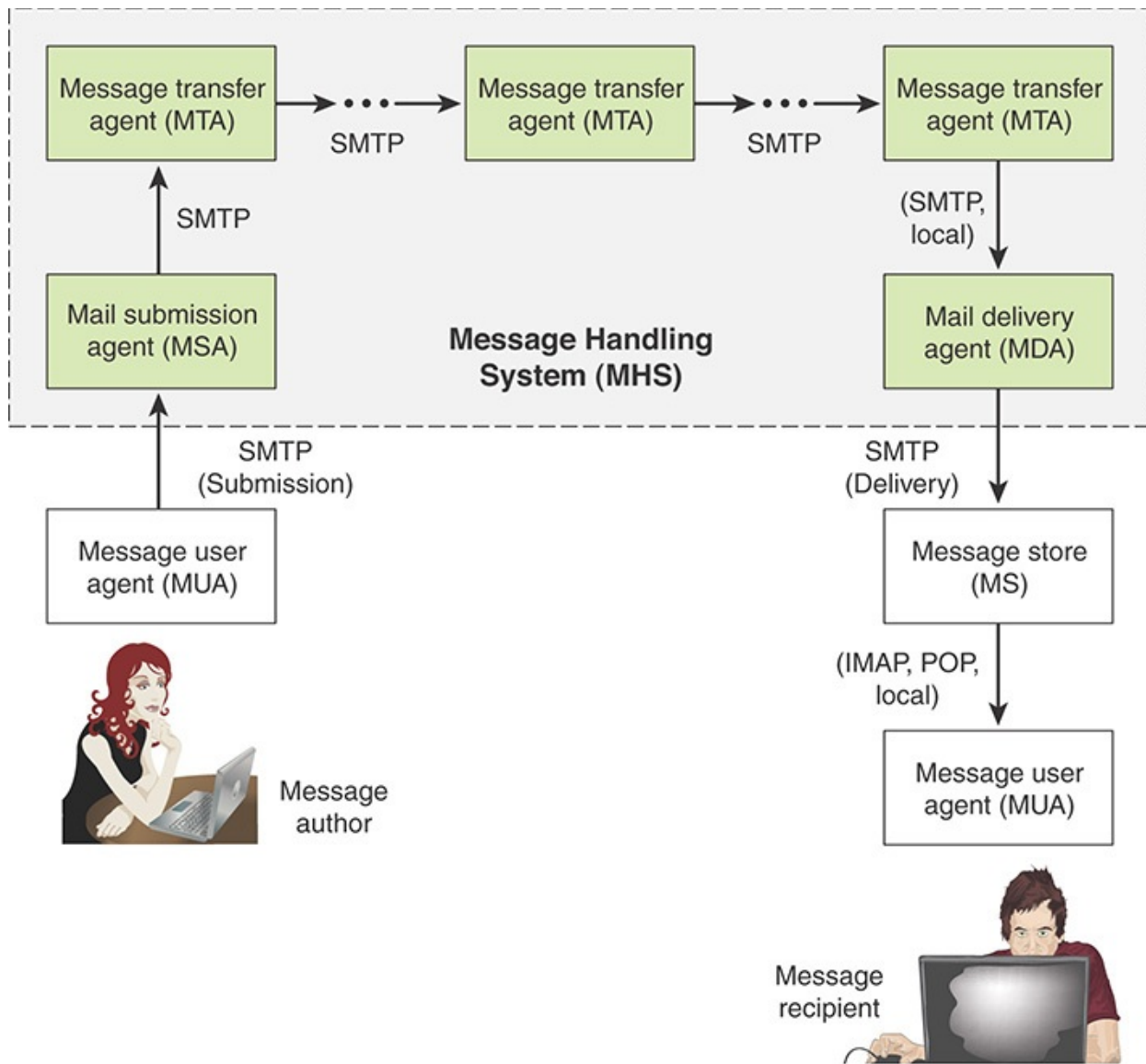
FIGURE 12.9 Function Modules and Standardized Protocols Used Between Them in the Internet Mail Architecture
