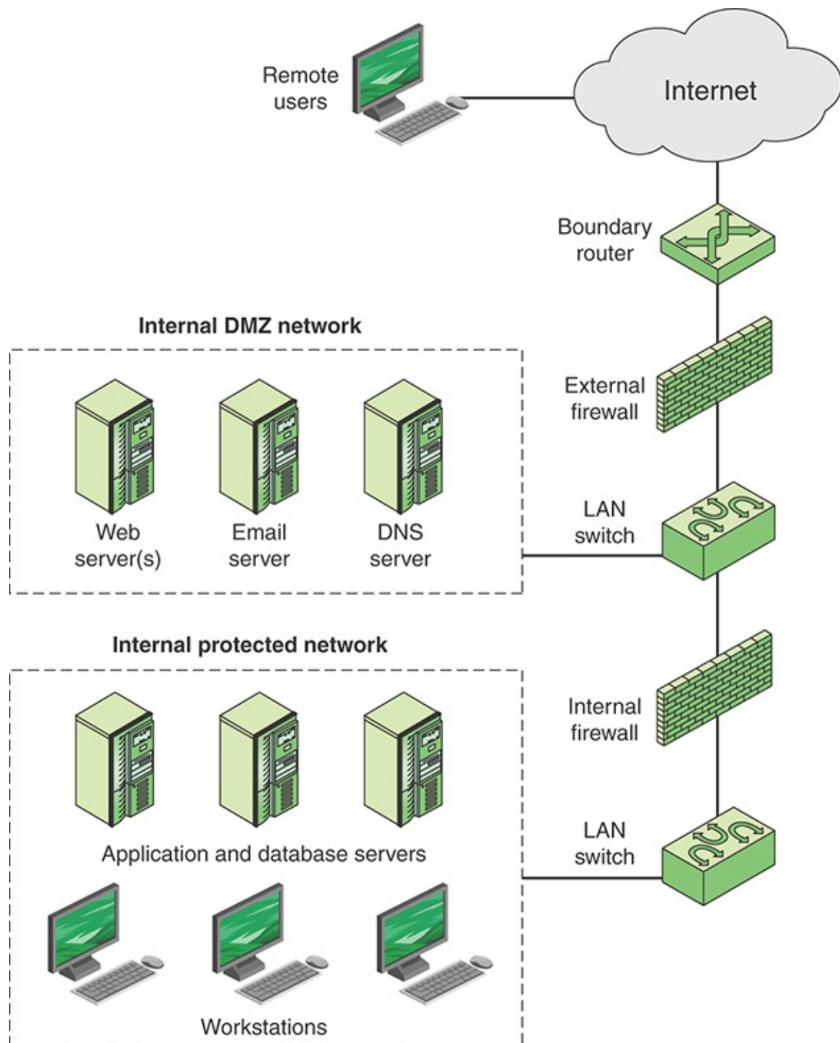
FIGURE 12.5 Firewall Configuration Example
