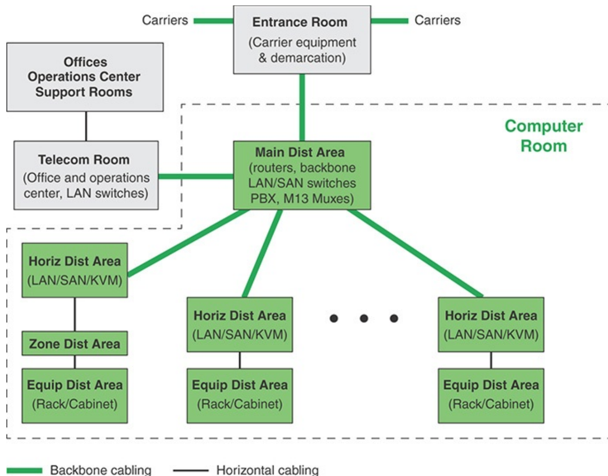
FIGURE 12.8 TIA-942-Compliant Data Center Showing Key Functional Areas
