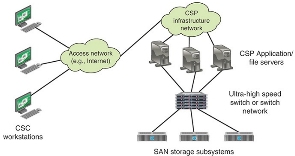
(a) Configuration with storage area network (SAN)
