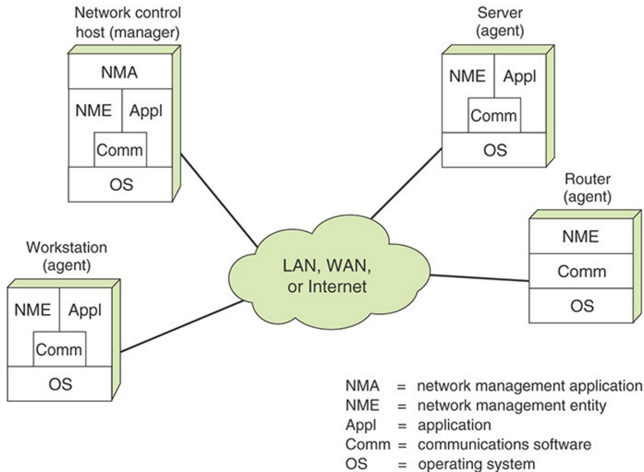
FIGURE 12.1 Components of a Network Management System
