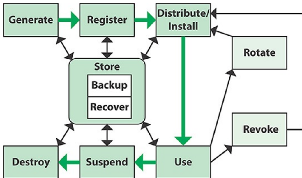
FIGURE 14.14 Cryptographic Key Life Cycle
