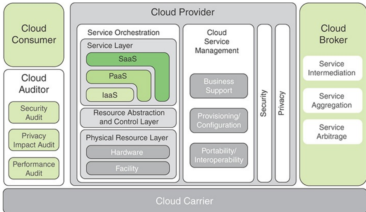
FIGURE 13.9 NIST Cloud Computing Reference Architecture
