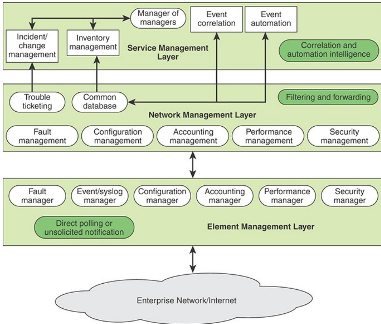
FIGURE 12.3 Network Management System Logical Architecture
