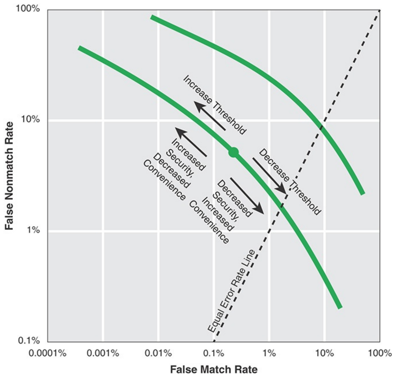
FIGURE 10.10 Idealized Biometric Measurement Operating Characteristic Curves (Log-Log Scale)
