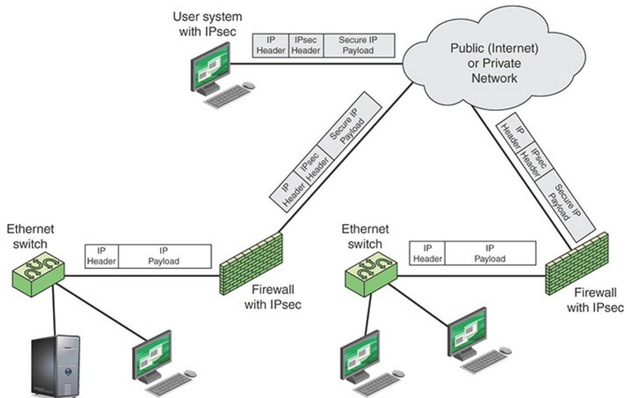
FIGURE 12.7 A VPN Security Scenario
